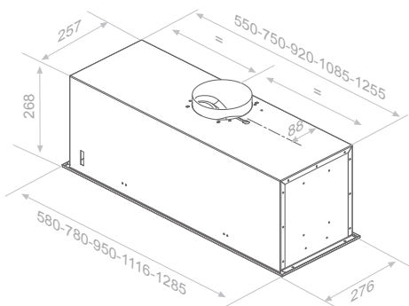
Medidas Encastre Dimensions Encastrement Built in Sizes
